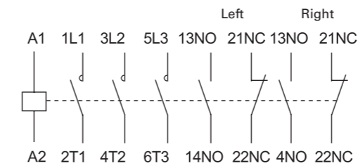
HDC3 185~630 with 2NO+2NC Auxiliary Contact
