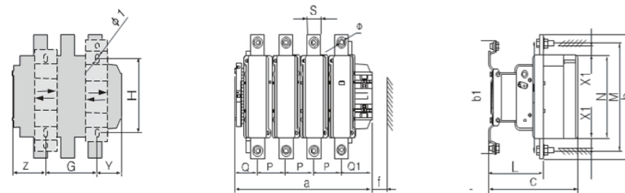
HJX2-F115~800 Overall Dimensions and Mounting Figures
