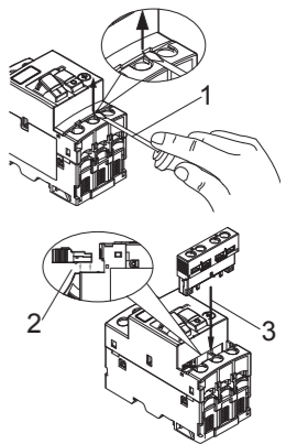
Installation of HAE11 or HAE20
