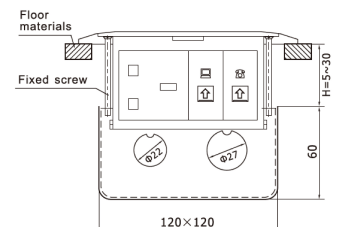
F. G. H>30mm can use longer fixing screws.
