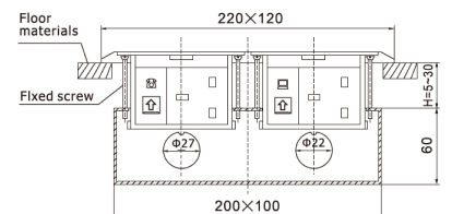
F. G. H>30mm can use longer fixing screws.
